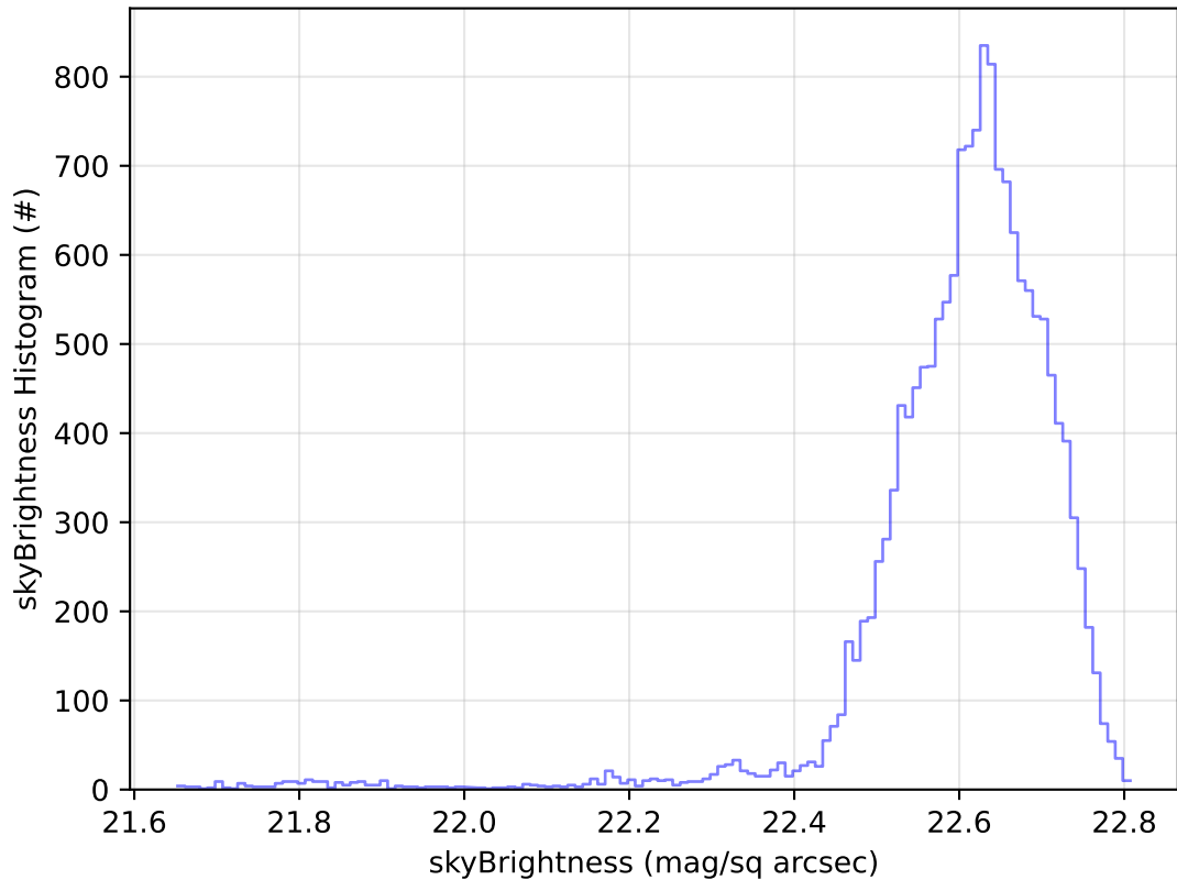
roll_uniform_early_half_mjdp0_v3.4_10yrs Yr 1 u band: skyBrightness Histogram
