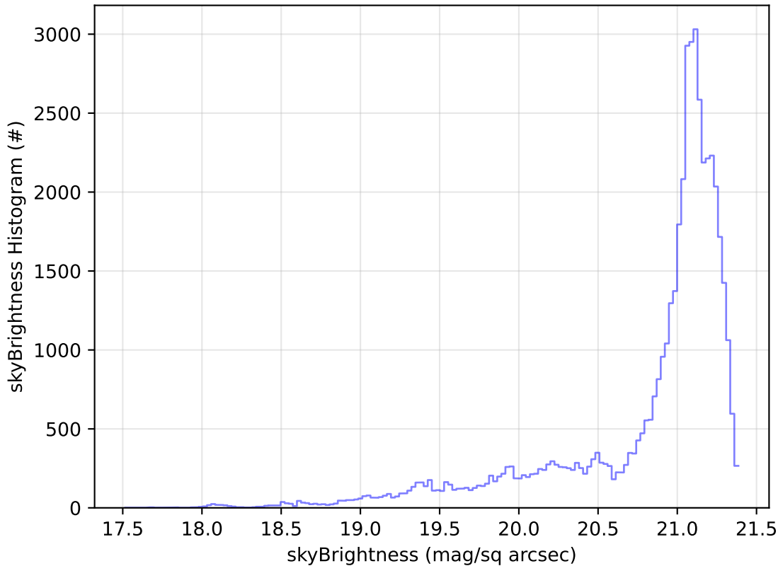
roll_uniform_early_half_mjdp0_v3.4_10yrs Yr 1 r band: skyBrightness Histogram
