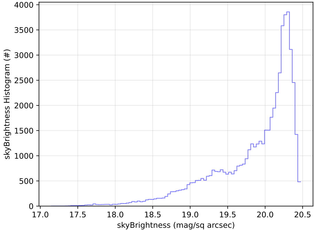
roll_uniform_early_half_mjdp0_v3.4_10yrs Yr 1 i band: skyBrightness Histogram
