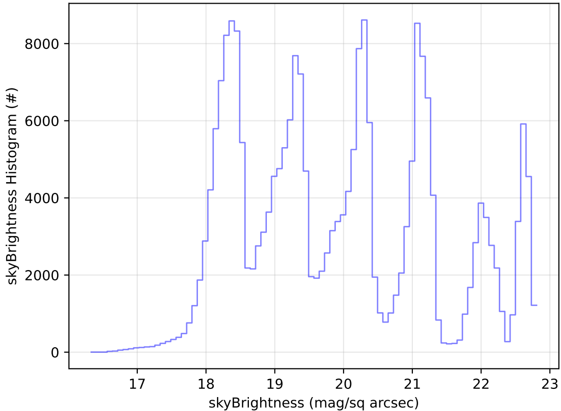
roll_uniform_early_half_mjdp0_v3.4_10yrs Yr 1 all bands: skyBrightness Histogram
