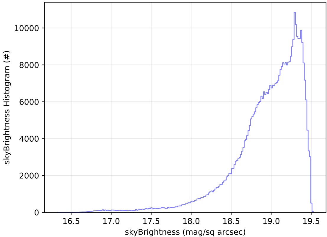
roll_uniform_early_half_mjdp0_v3.4_10yrs WFD z band: skyBrightness Histogram
