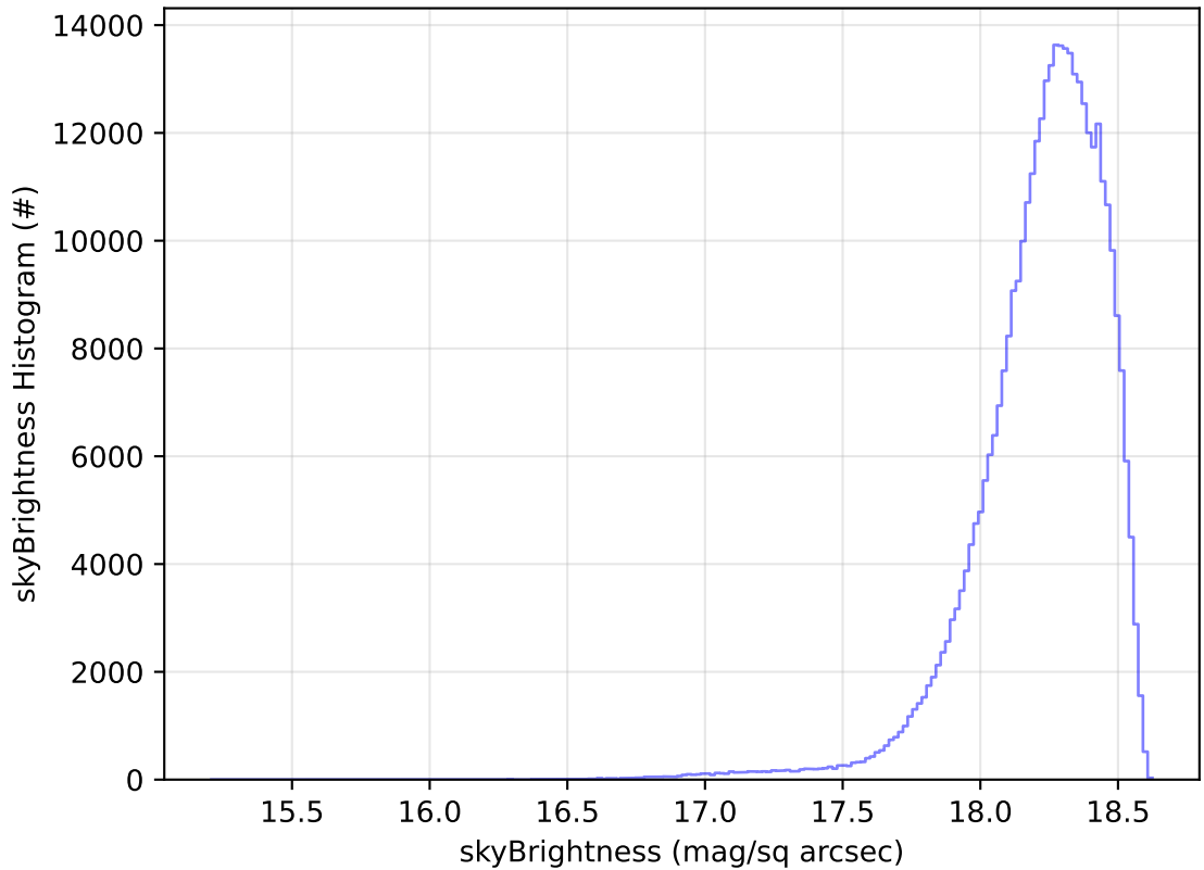
roll_uniform_early_half_mjdp0_v3.4_10yrs WFD y band: skyBrightness Histogram
