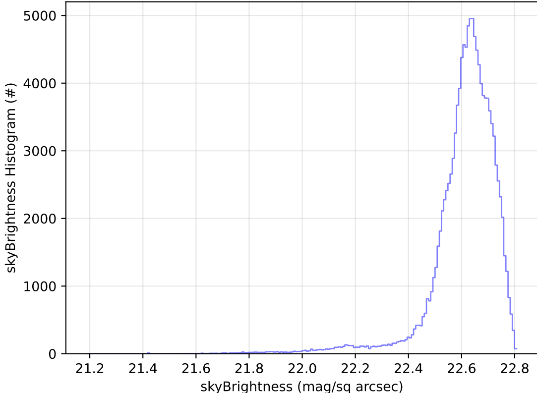
roll_uniform_early_half_mjdp0_v3.4_10yrs WFD u band: skyBrightness Histogram
