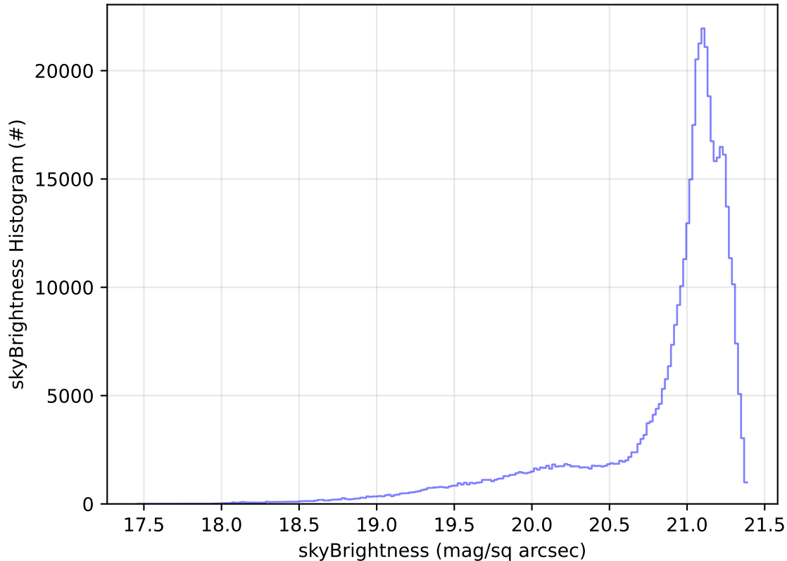
roll_uniform_early_half_mjdp0_v3.4_10yrs WFD r band: skyBrightness Histogram
