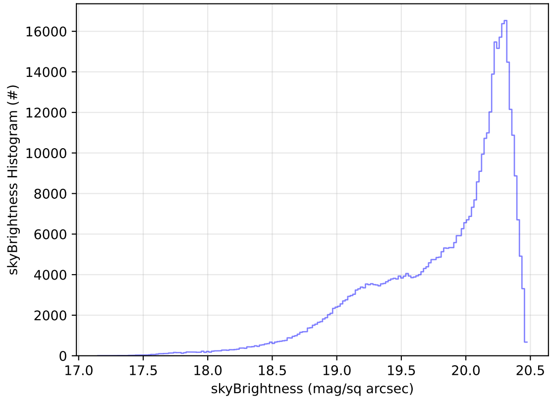
roll_uniform_early_half_mjdp0_v3.4_10yrs WFD i band: skyBrightness Histogram
