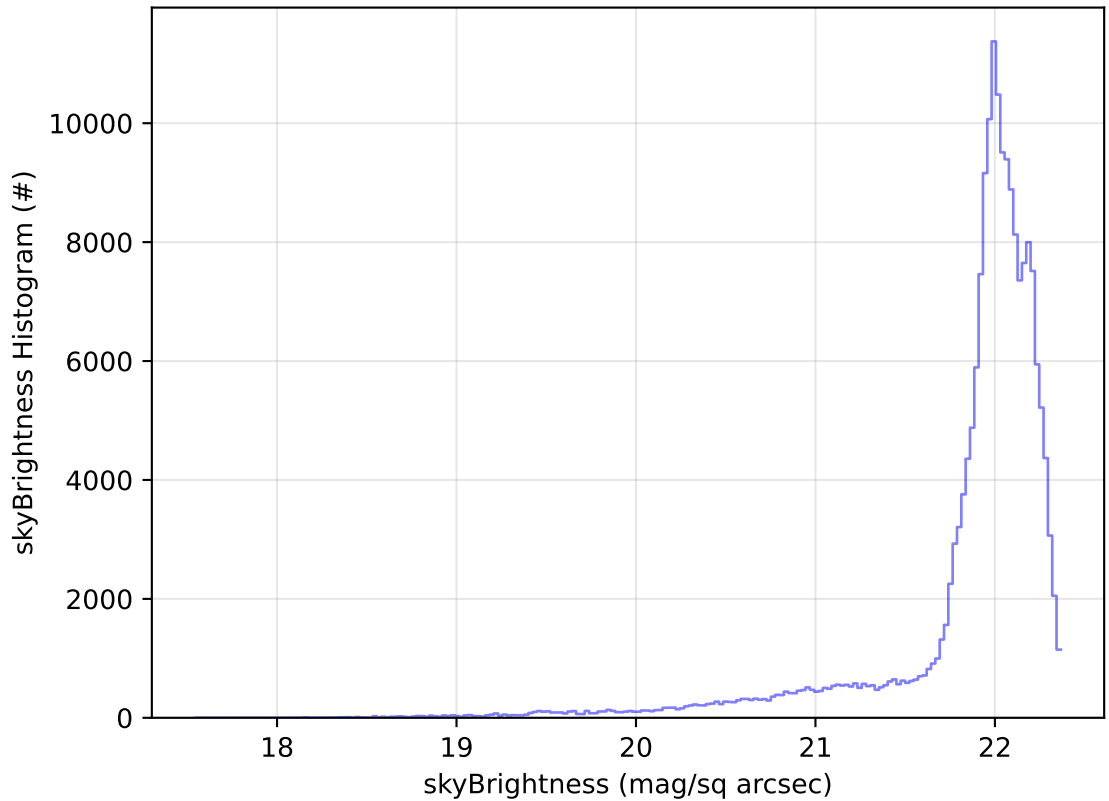
roll_uniform_early_half_mjdp0_v3.4_10yrs WFD g band: skyBrightness Histogram
