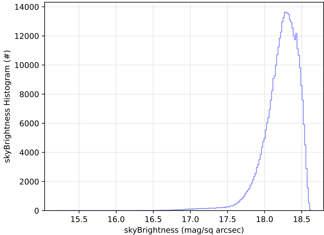
roll_uniform_early_half_mjdp0_v3.4_10yrs All sky y band: skyBrightness Histogram
