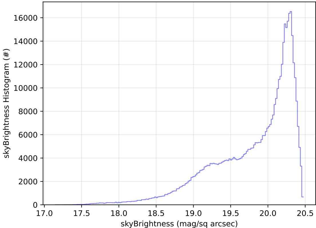
roll_uniform_early_half_mjdp0_v3.4_10yrs All sky i band: skyBrightness Histogram
