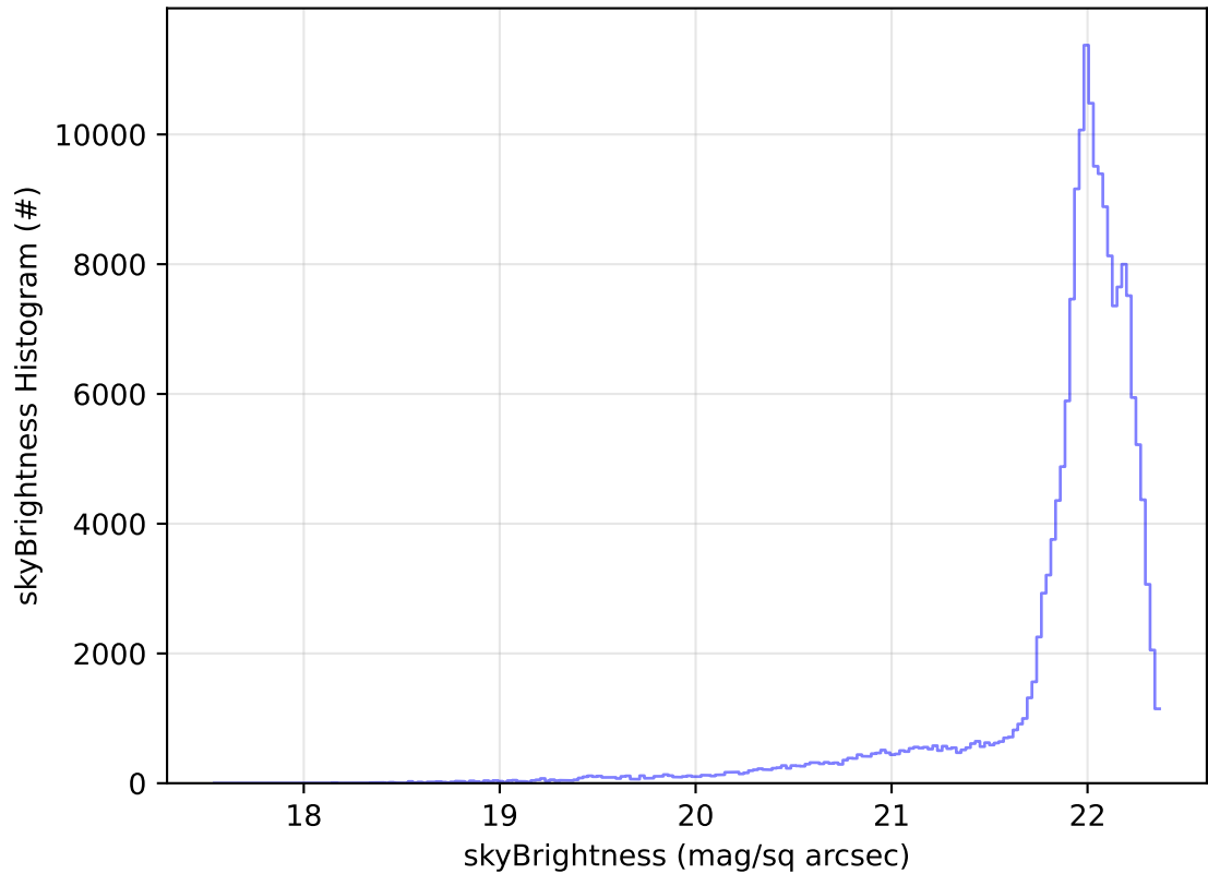
roll_uniform_early_half_mjdp0_v3.4_10yrs All sky g band: skyBrightness Histogram
