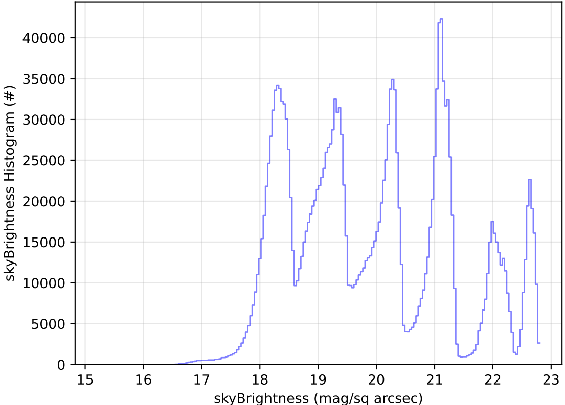
roll_uniform_early_half_mjdp0_v3.4_10yrs All sky all bands: skyBrightness Histogram
