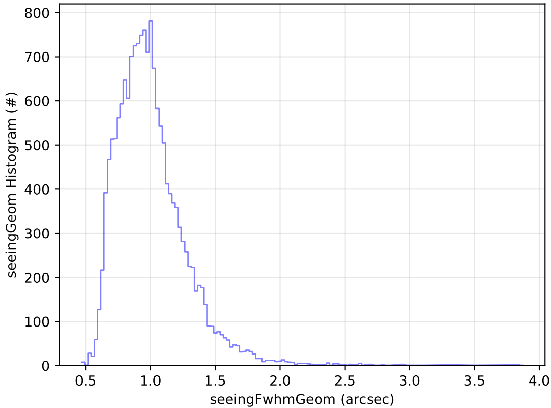
roll_uniform_early_half_mjdp0_v3.4_10yrs Yr 1 u band: seeingGeom Histogram
