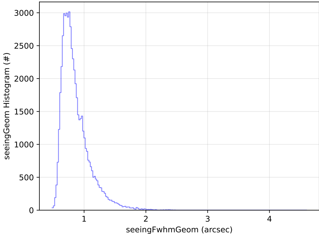
roll_uniform_early_half_mjdp0_v3.4_10yrs Yr 1 i band: seeingGeom Histogram
