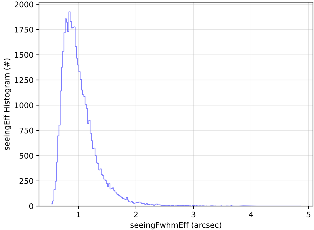
roll_uniform_early_half_mjdp0_v3.4_10yrs Yr 1 z band: seeingEff Histogram
