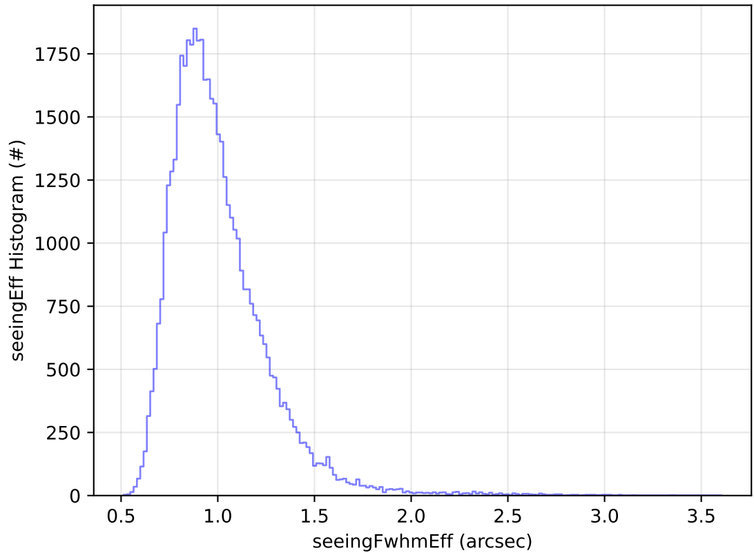
roll_uniform_early_half_mjdp0_v3.4_10yrs Yr 1 y band: seeingEff Histogram
