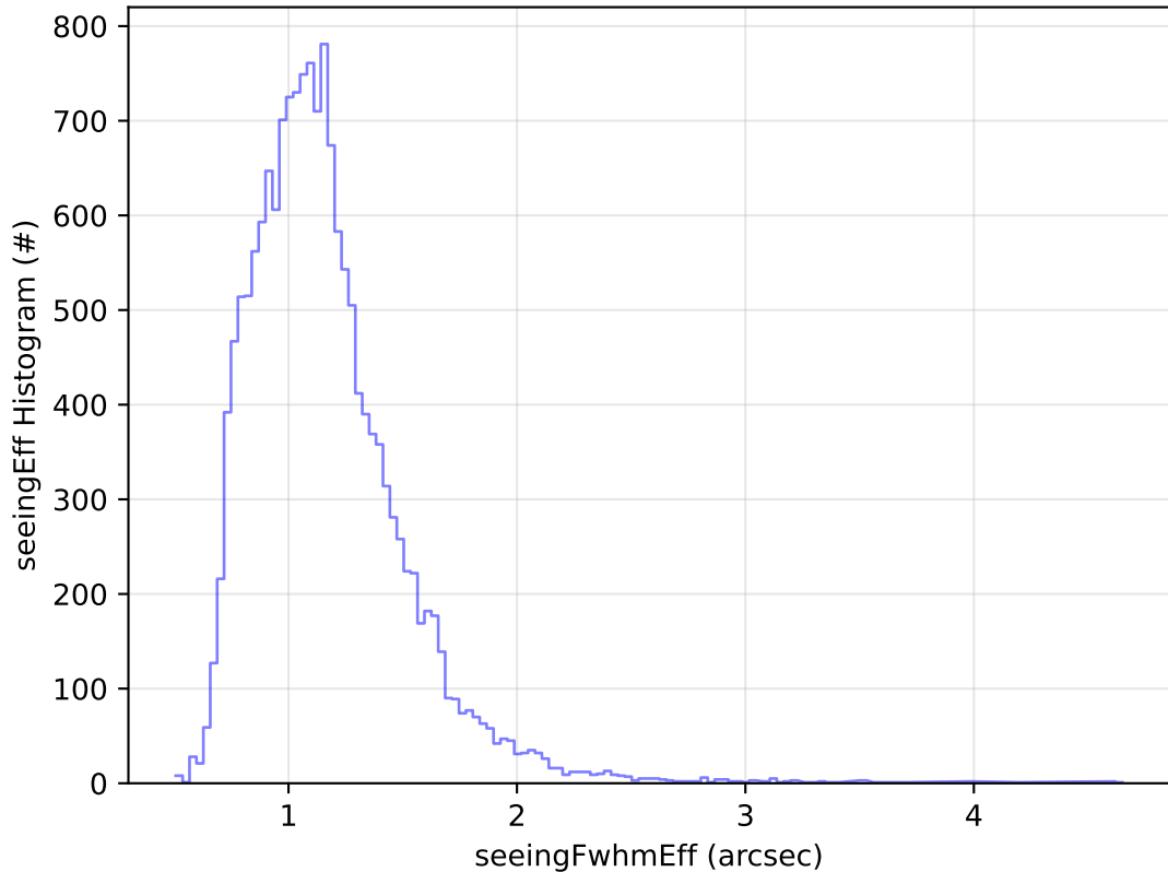
roll_uniform_early_half_mjdp0_v3.4_10yrs Yr 1 u band: seeingEff Histogram
