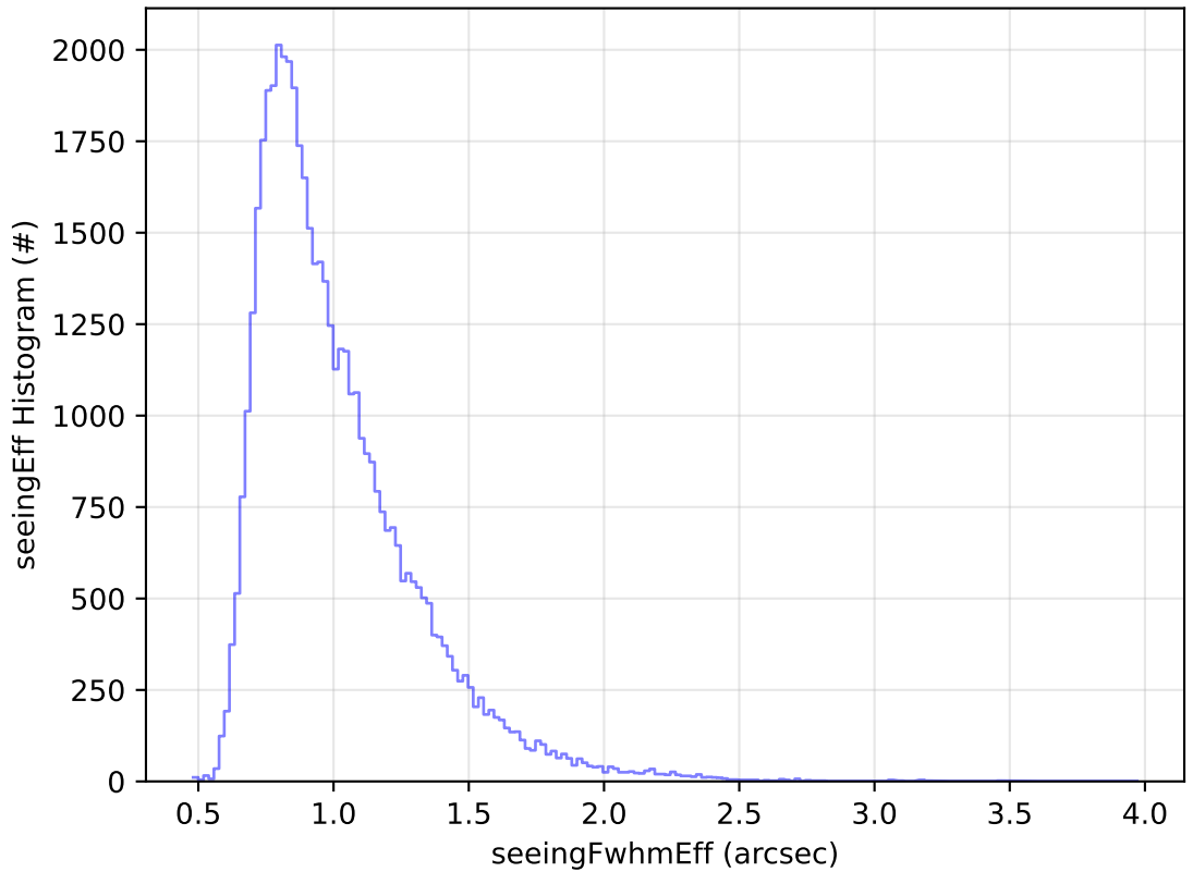
roll_uniform_early_half_mjdp0_v3.4_10yrs Yr 1 r band: seeingEff Histogram
