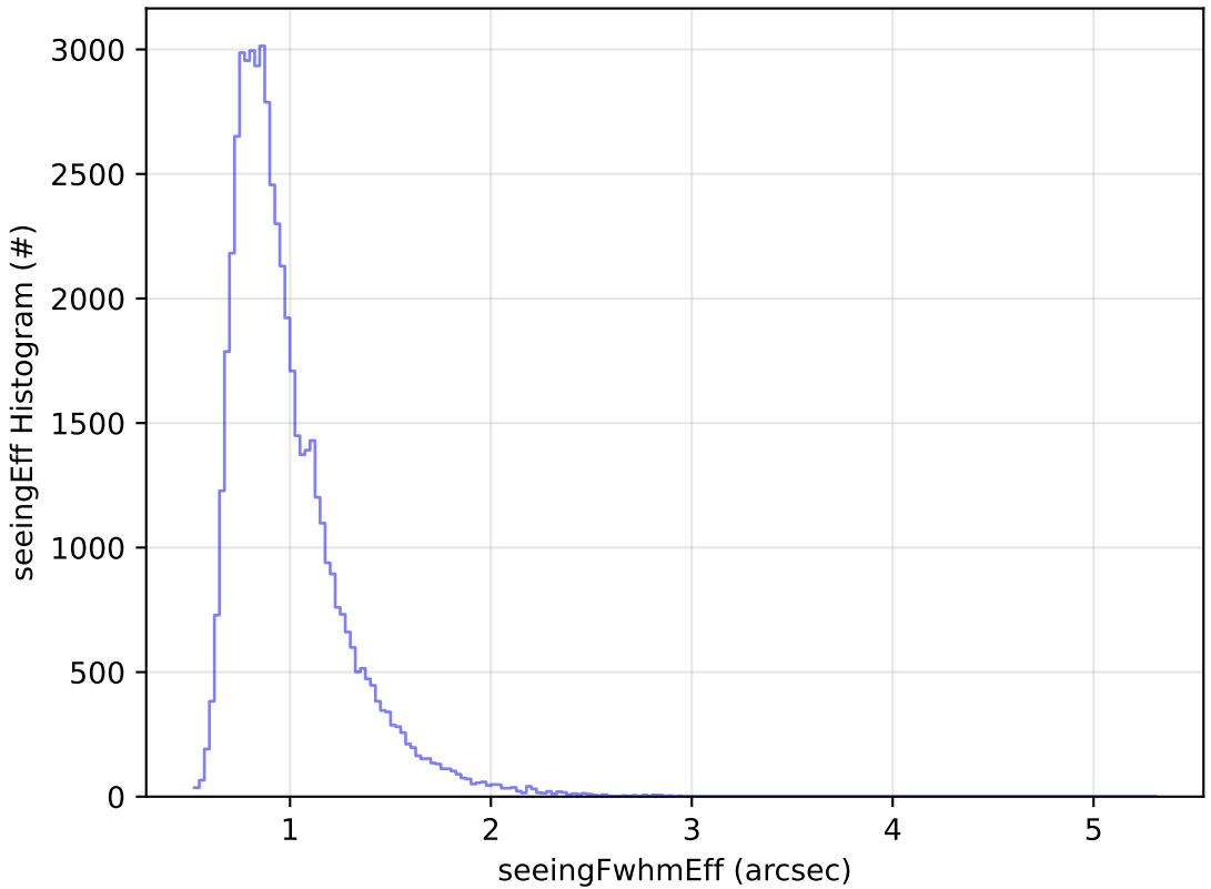
roll_uniform_early_half_mjdp0_v3.4_10yrs Yr 1 i band: seeingEff Histogram
