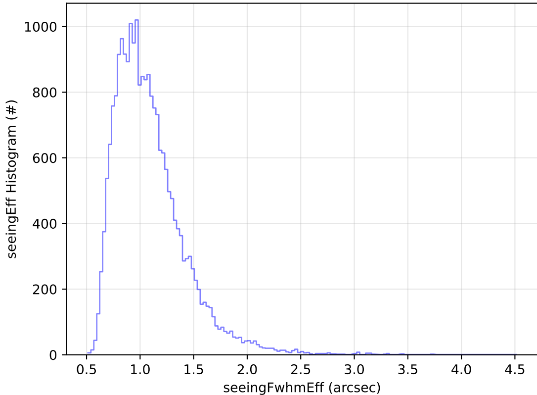
roll_uniform_early_half_mjdp0_v3.4_10yrs Yr 1 g band: seeingEff Histogram
