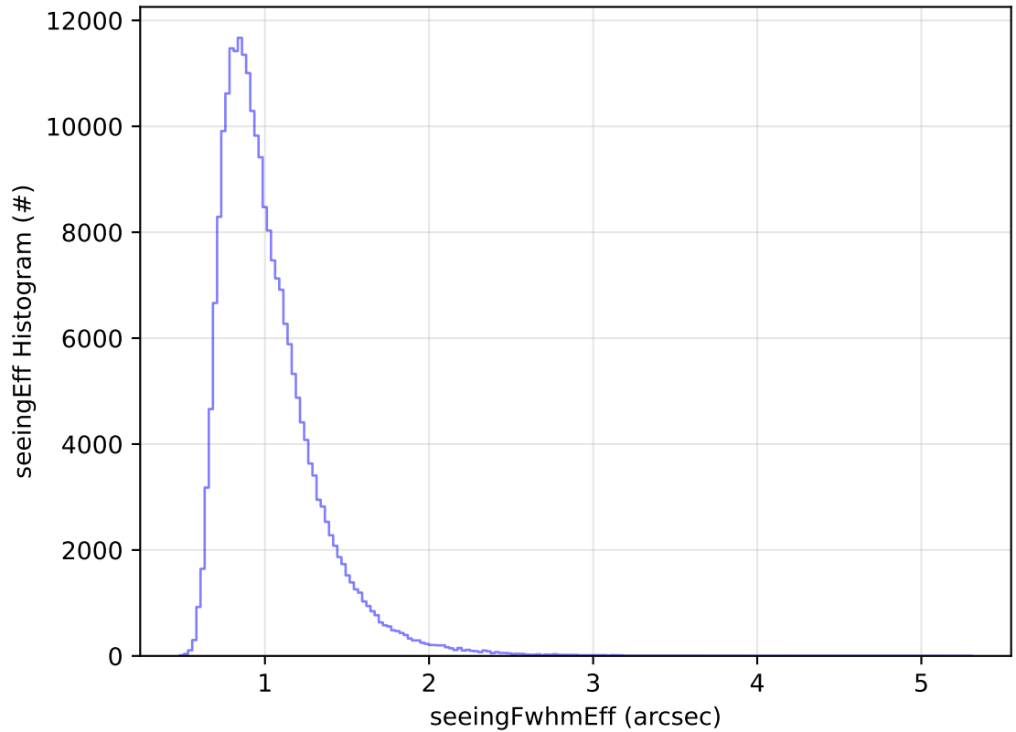
roll_uniform_early_half_mjdp0_v3.4_10yrs Yr 1 all bands: seeingEff Histogram
