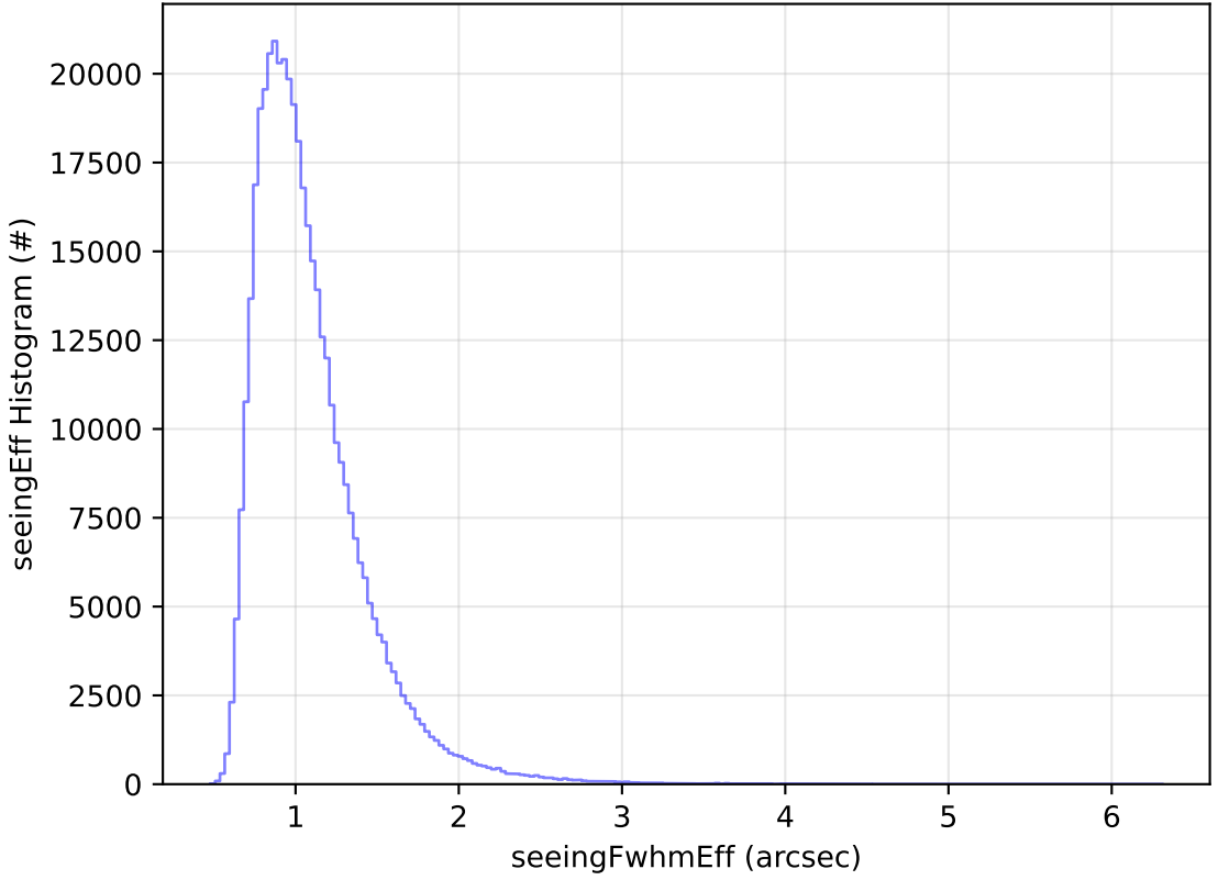
roll_uniform_early_half_mjdp0_v3.4_10yrs WFD z band: seeingEff Histogram
