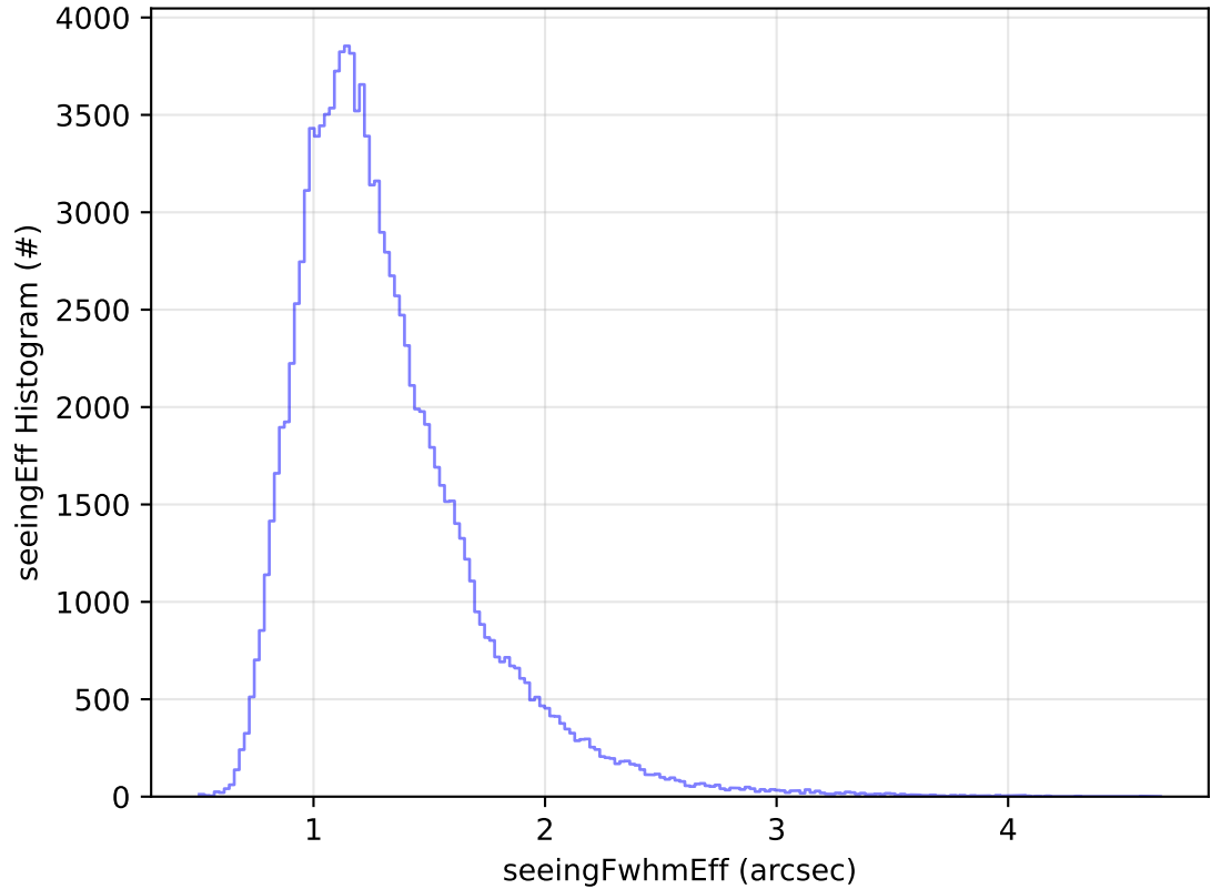
roll_uniform_early_half_mjdp0_v3.4_10yrs WFD u band: seeingEff Histogram
