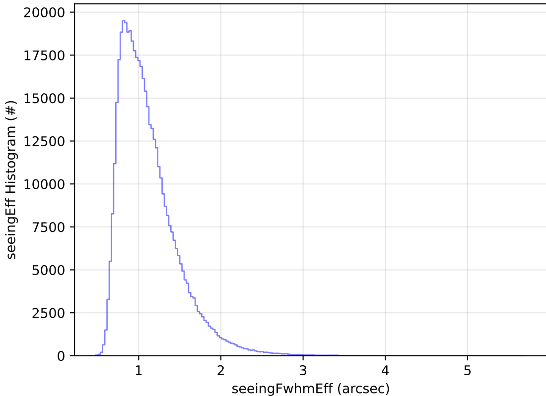
roll_uniform_early_half_mjdp0_v3.4_10yrs WFD r band: seeingEff Histogram
