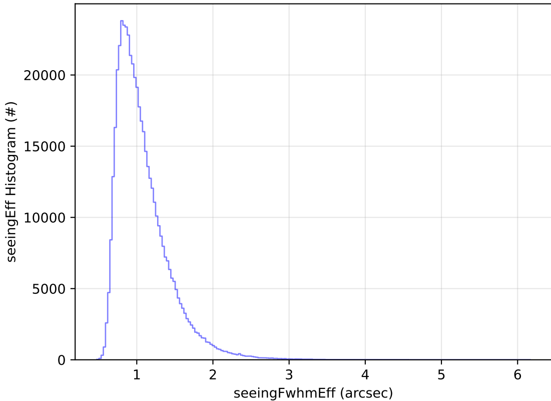
roll_uniform_early_half_mjdp0_v3.4_10yrs WFD i band: seeingEff Histogram
