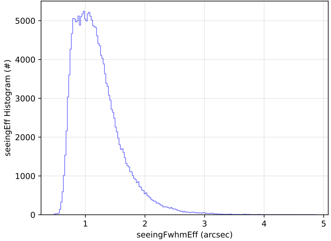
roll_uniform_early_half_mjdp0_v3.4_10yrs WFD g band: seeingEff Histogram
