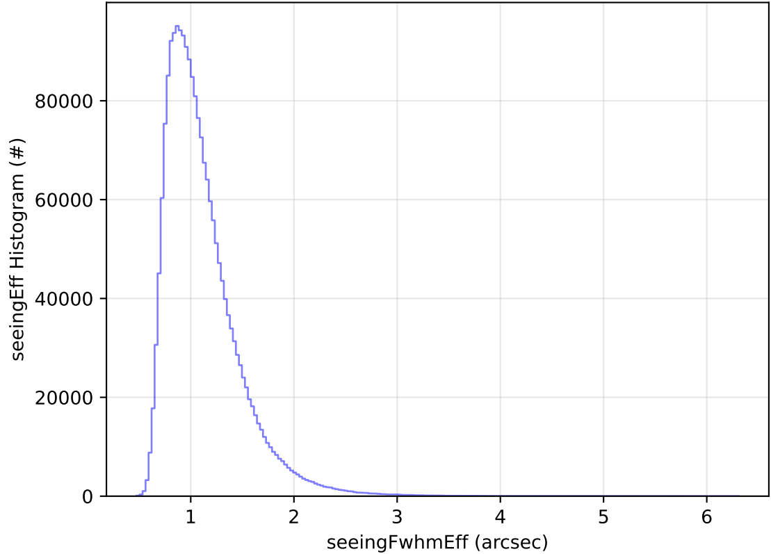
roll_uniform_early_half_mjdp0_v3.4_10yrs WFD all bands: seeingEff Histogram
