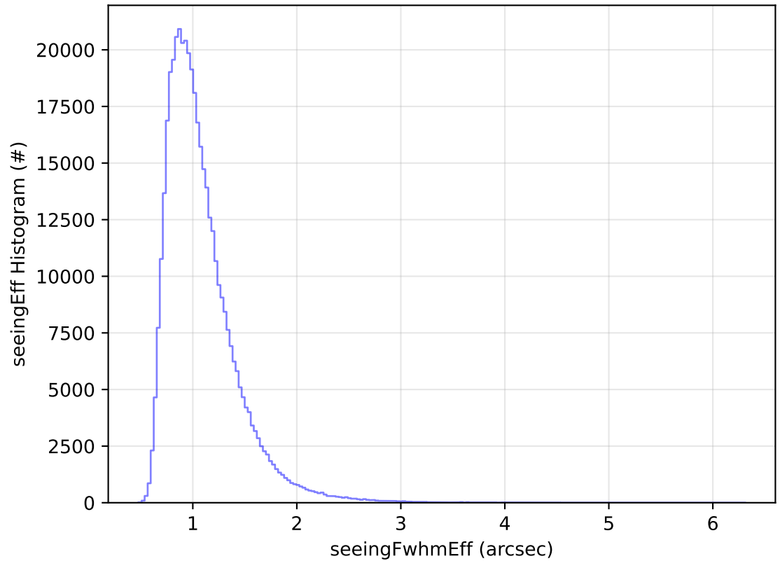
roll_uniform_early_half_mjdp0_v3.4_10yrs All sky z band: seeingEff Histogram
