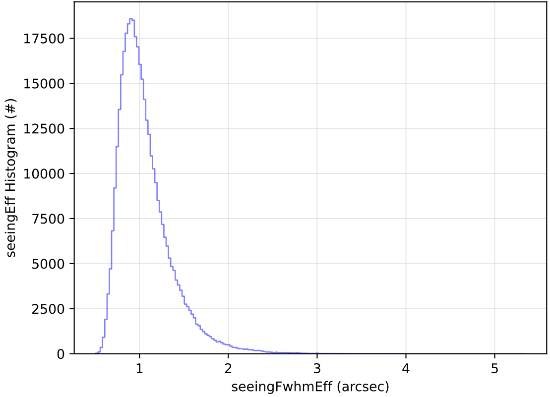
roll_uniform_early_half_mjdp0_v3.4_10yrs All sky y band: seeingEff Histogram
