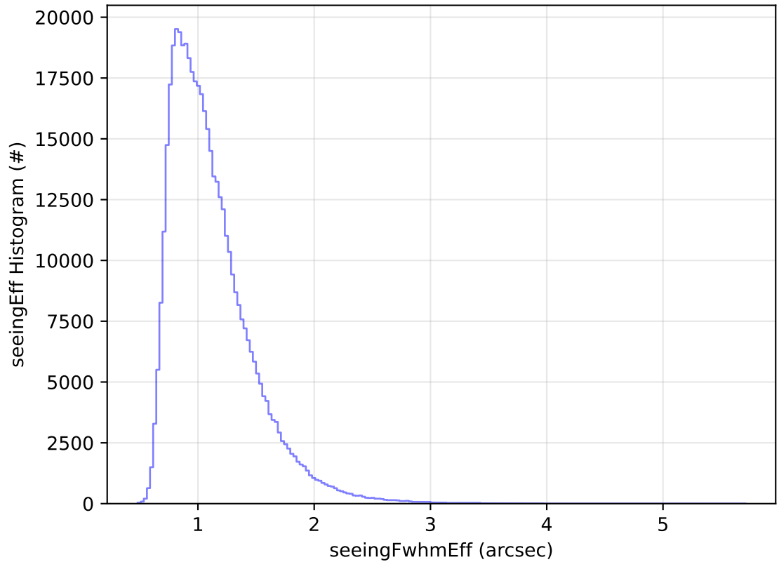
roll_uniform_early_half_mjdp0_v3.4_10yrs All sky r band: seeingEff Histogram
