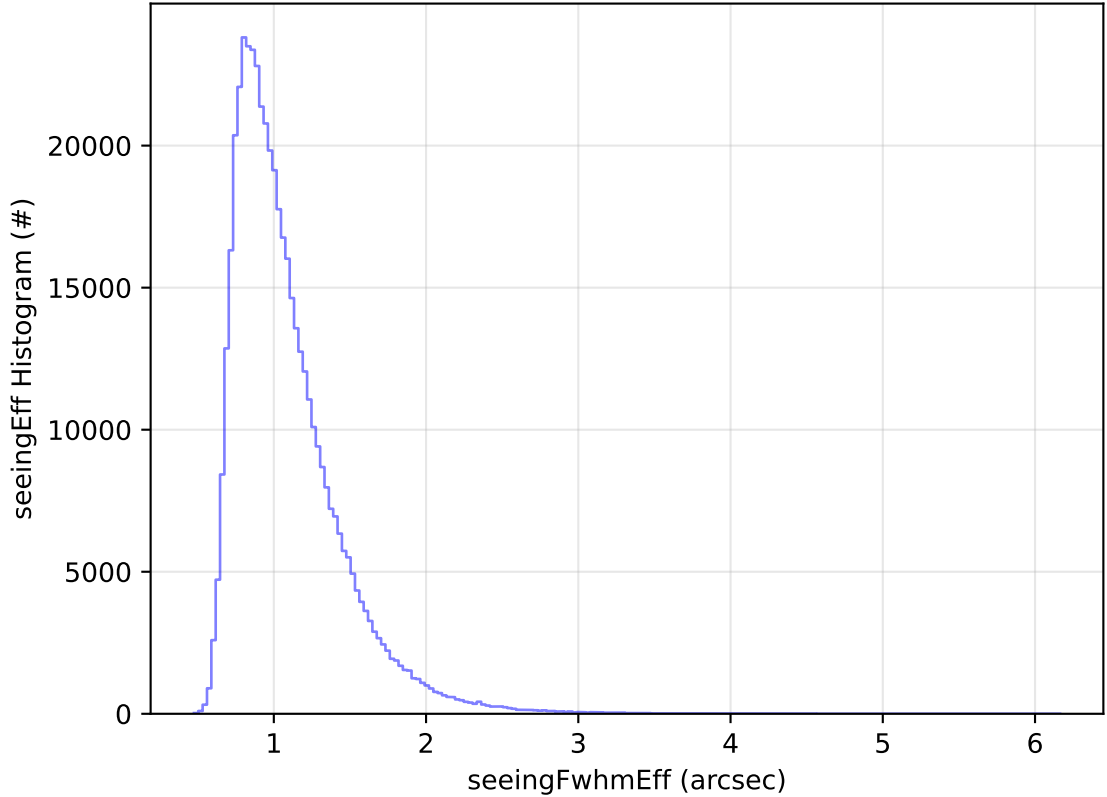
roll_uniform_early_half_mjdp0_v3.4_10yrs All sky i band: seeingEff Histogram
