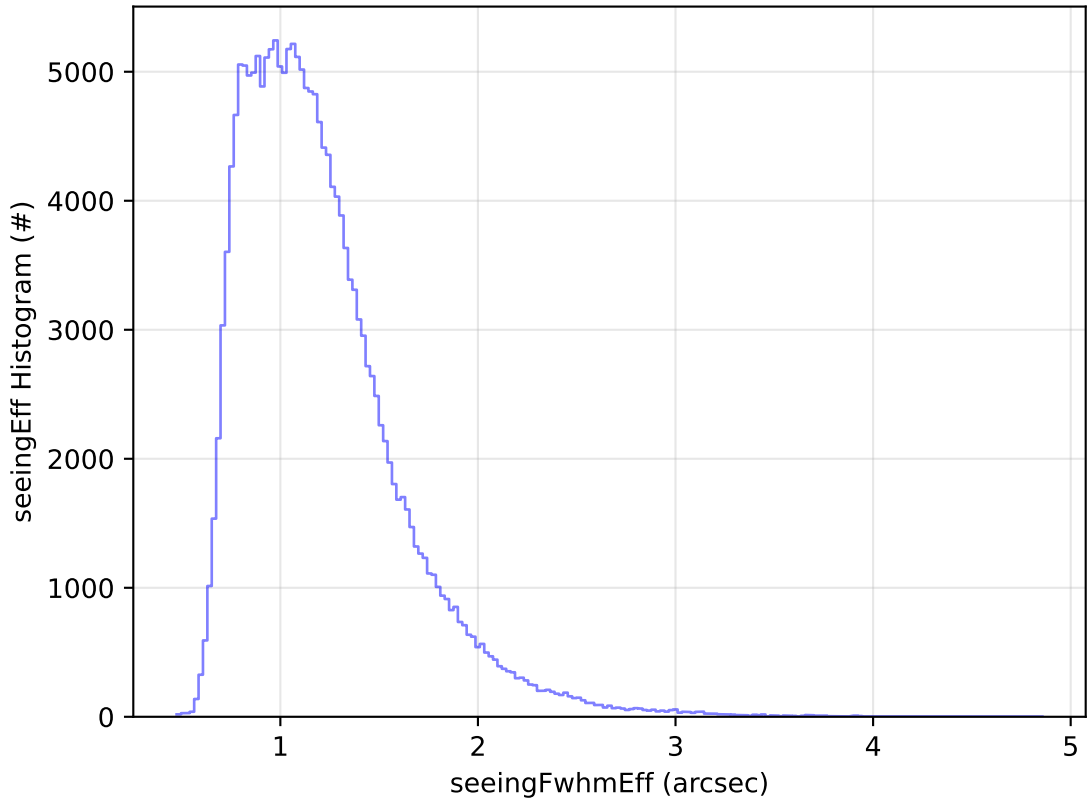
roll_uniform_early_half_mjdp0_v3.4_10yrs All sky g band: seeingEff Histogram
