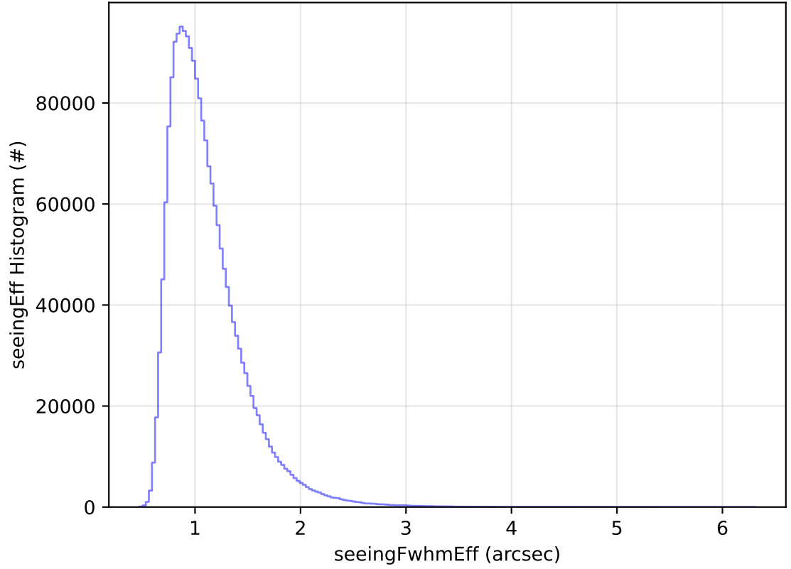
roll_uniform_early_half_mjdp0_v3.4_10yrs All sky all bands: seeingEff Histogram
