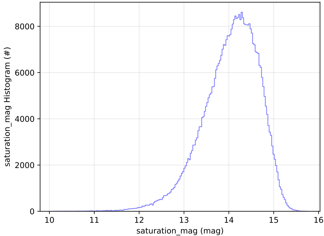
roll_uniform_early_half_mjdp0_v3.4_10yrs WFD z band: saturation_mag Histogram
