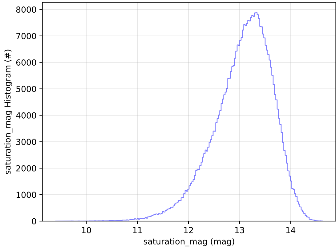
roll_uniform_early_half_mjdp0_v3.4_10yrs WFD y band: saturation_mag Histogram
