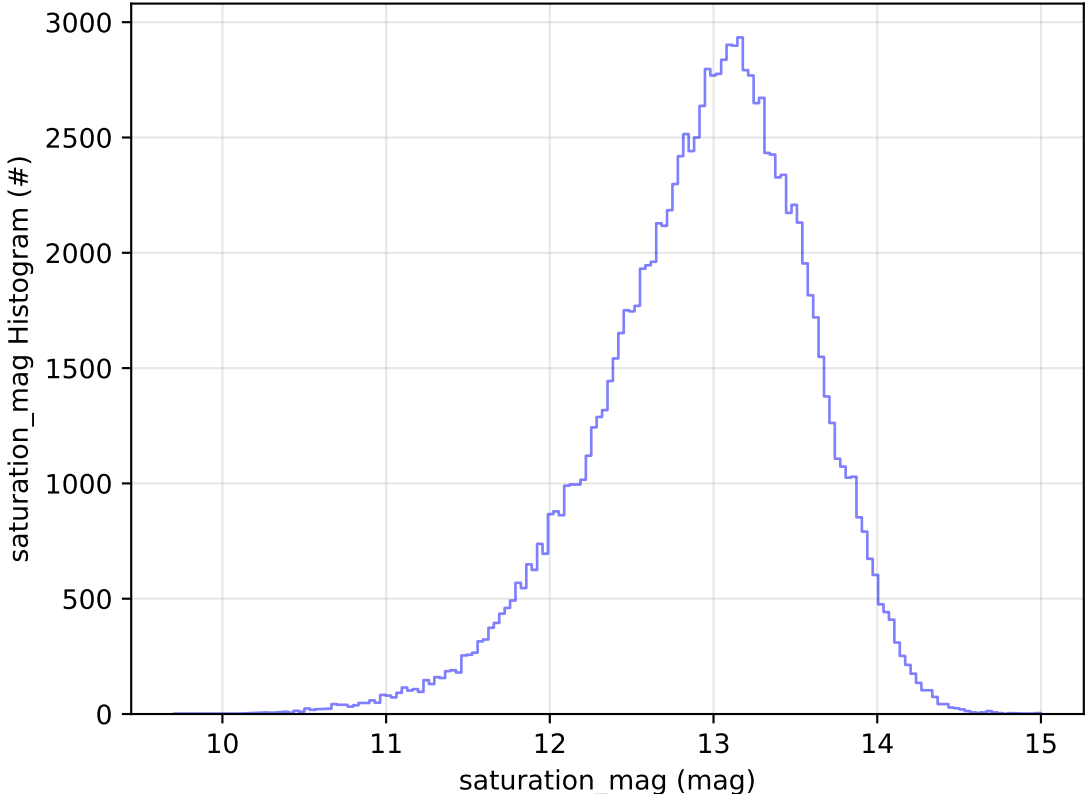
roll_uniform_early_half_mjdp0_v3.4_10yrs WFD u band: saturation_mag Histogram
