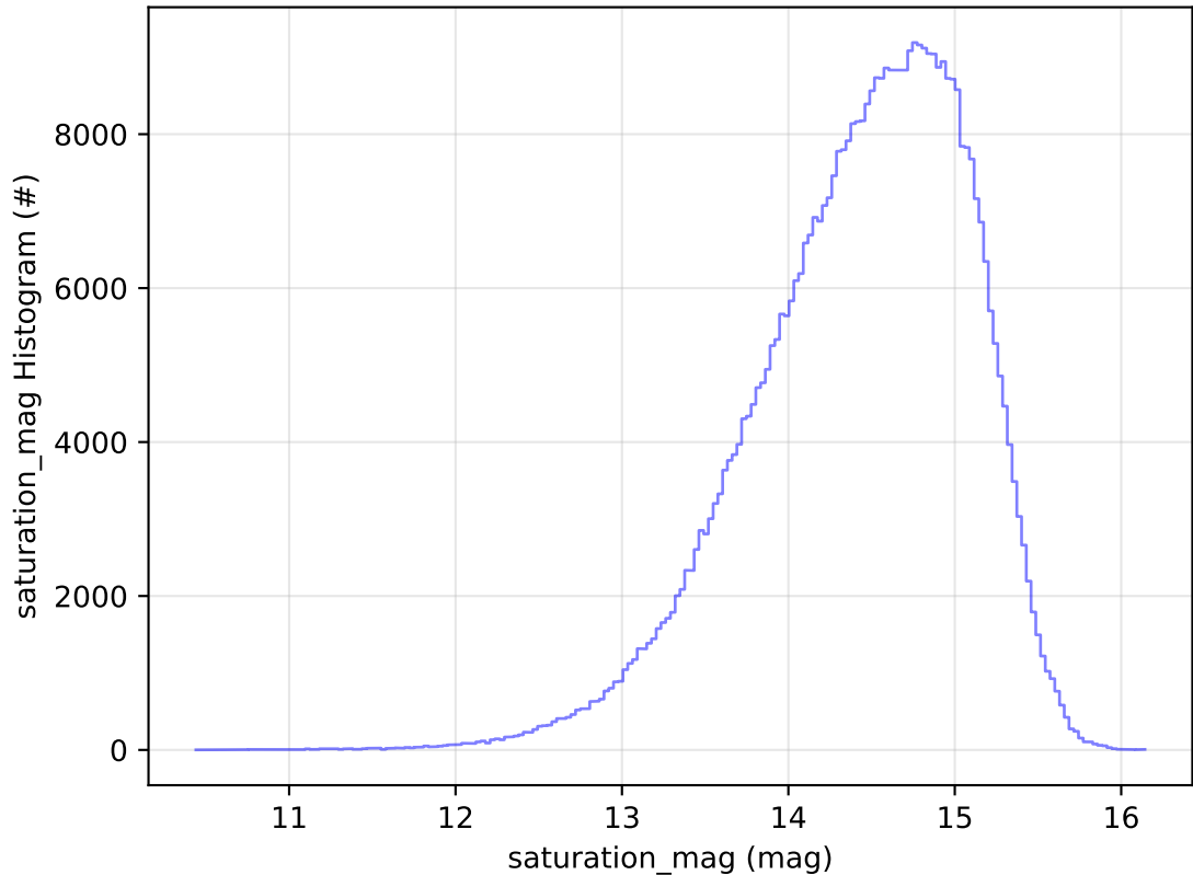
roll_uniform_early_half_mjdp0_v3.4_10yrs WFD i band: saturation_mag Histogram
