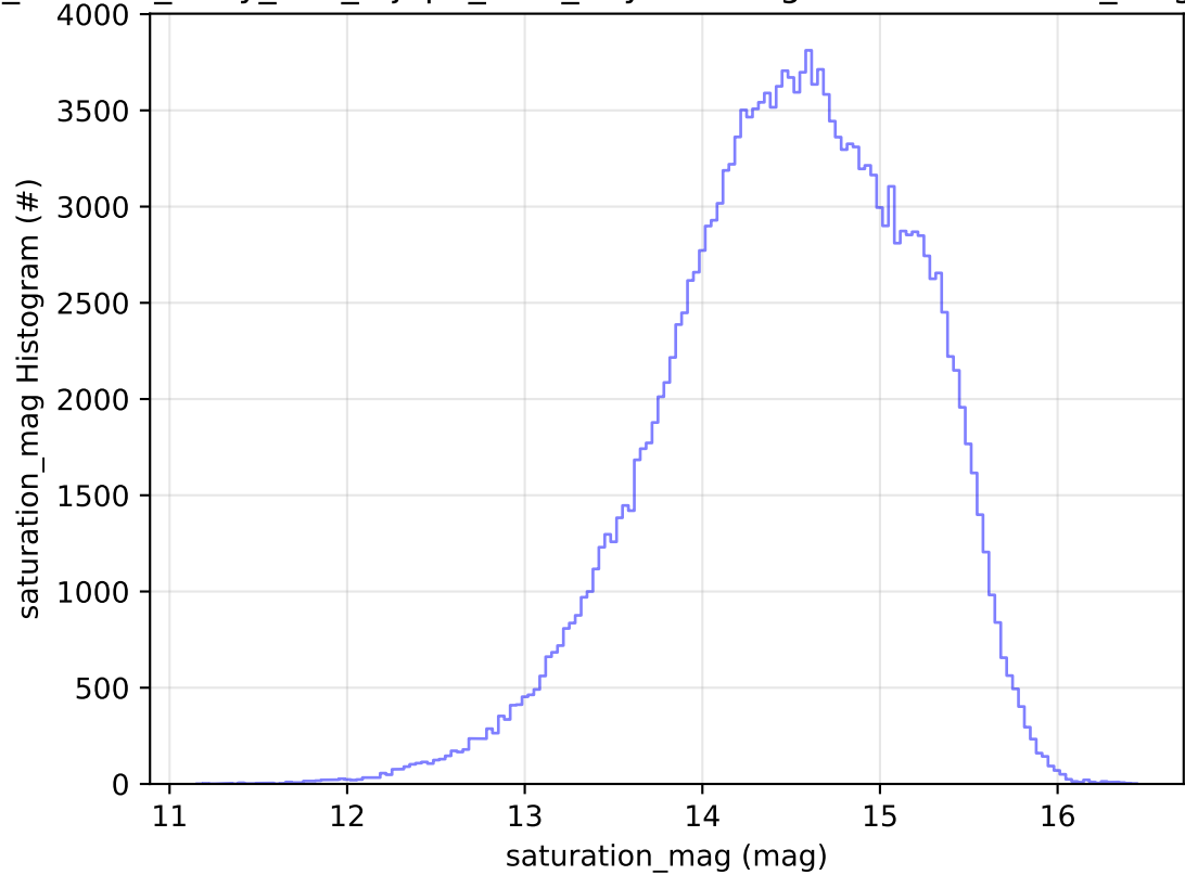
roll_uniform_early_half_mjdp0_v3.4_10yrs WFD g band: saturation_mag Histogram
