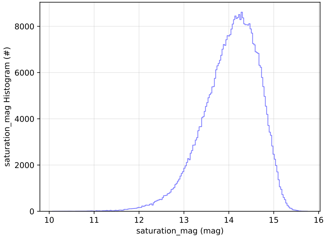
roll_uniform_early_half_mjdp0_v3.4_10yrs All sky z band: saturation_mag Histogram
