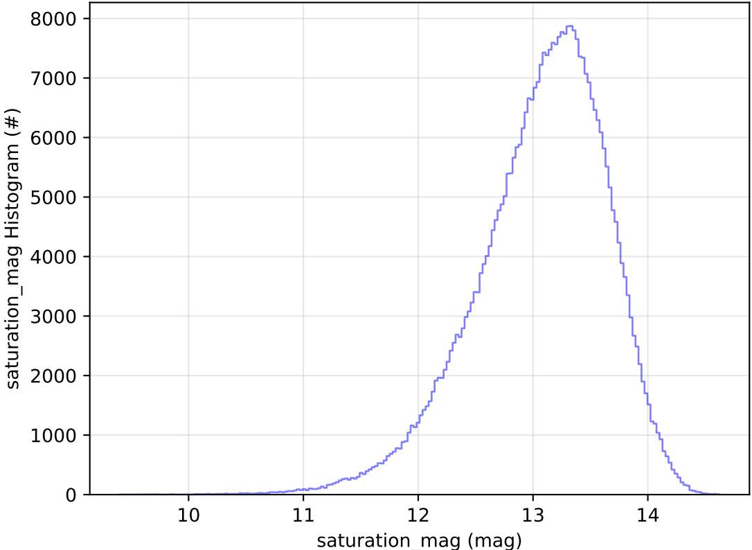
roll_uniform_early_half_mjdp0_v3.4_10yrs All sky y band: saturation_mag Histogram
