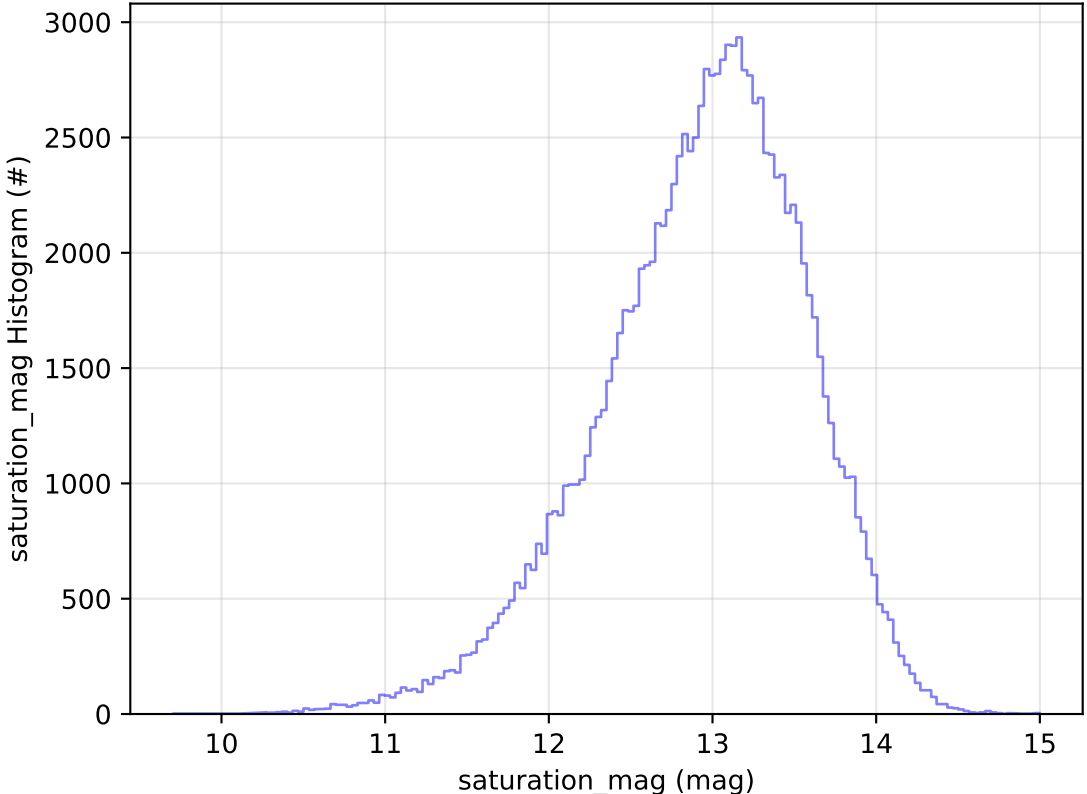
roll_uniform_early_half_mjdp0_v3.4_10yrs All sky u band: saturation_mag Histogram
