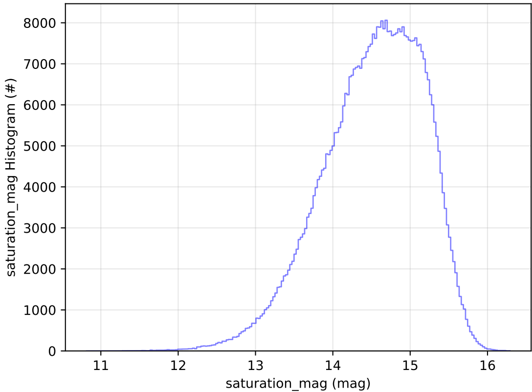
roll_uniform_early_half_mjdp0_v3.4_10yrs All sky r band: saturation_mag Histogram
