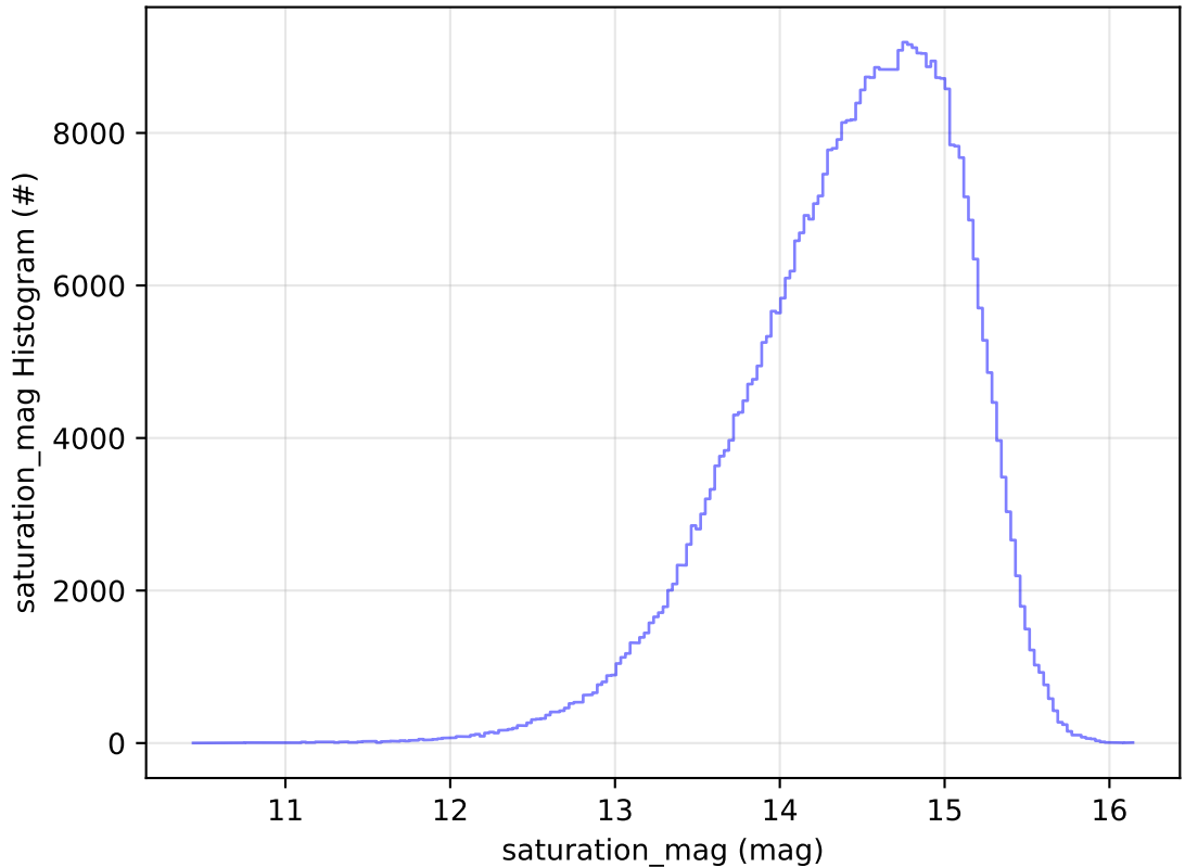
roll_uniform_early_half_mjdp0_v3.4_10yrs All sky i band: saturation_mag Histogram
