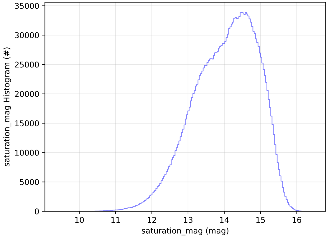
roll_uniform_early_half_mjdp0_v3.4_10yrs All sky all bands: saturation_mag Histogram
