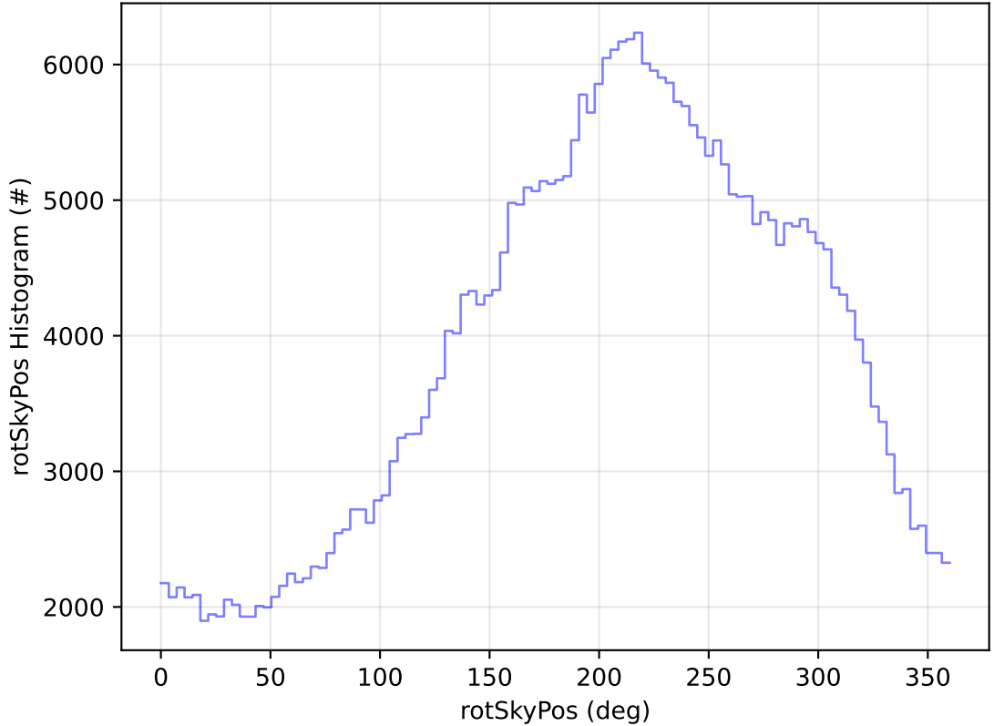
roll_uniform_early_half_mjdp0_v3.4_10yrs WFD y band: rotSkyPos Histogram
