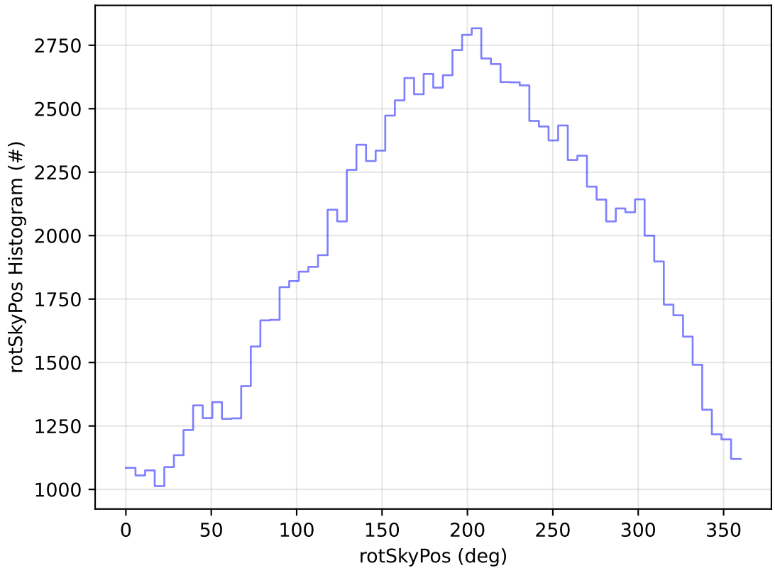
roll_uniform_early_half_mjdp0_v3.4_10yrs WFD u band: rotSkyPos Histogram
