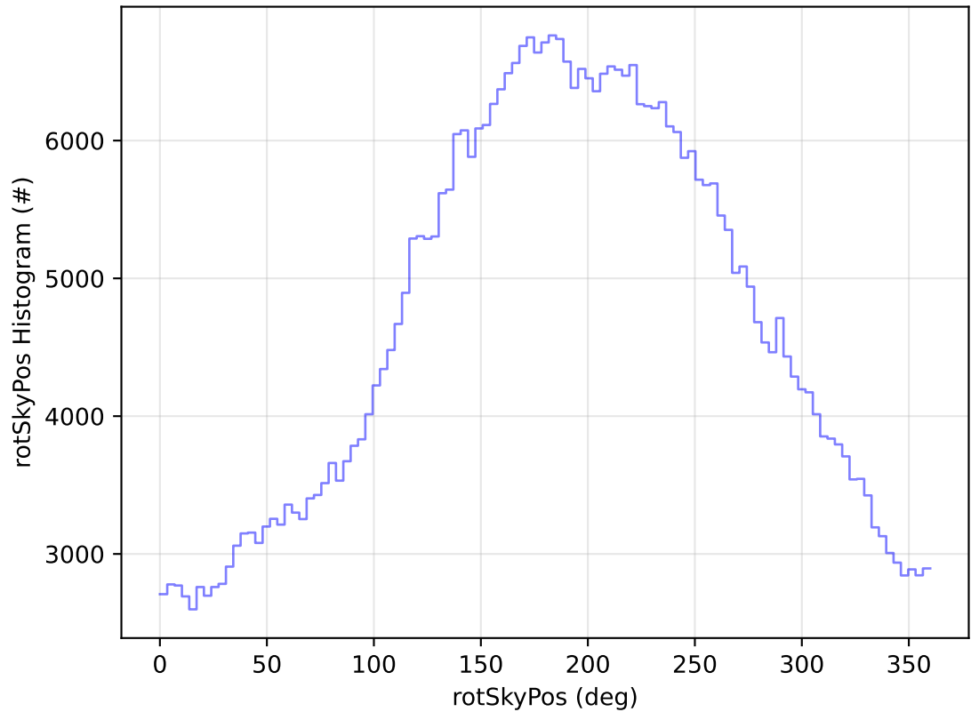
roll_uniform_early_half_mjdp0_v3.4_10yrs WFD r band: rotSkyPos Histogram
