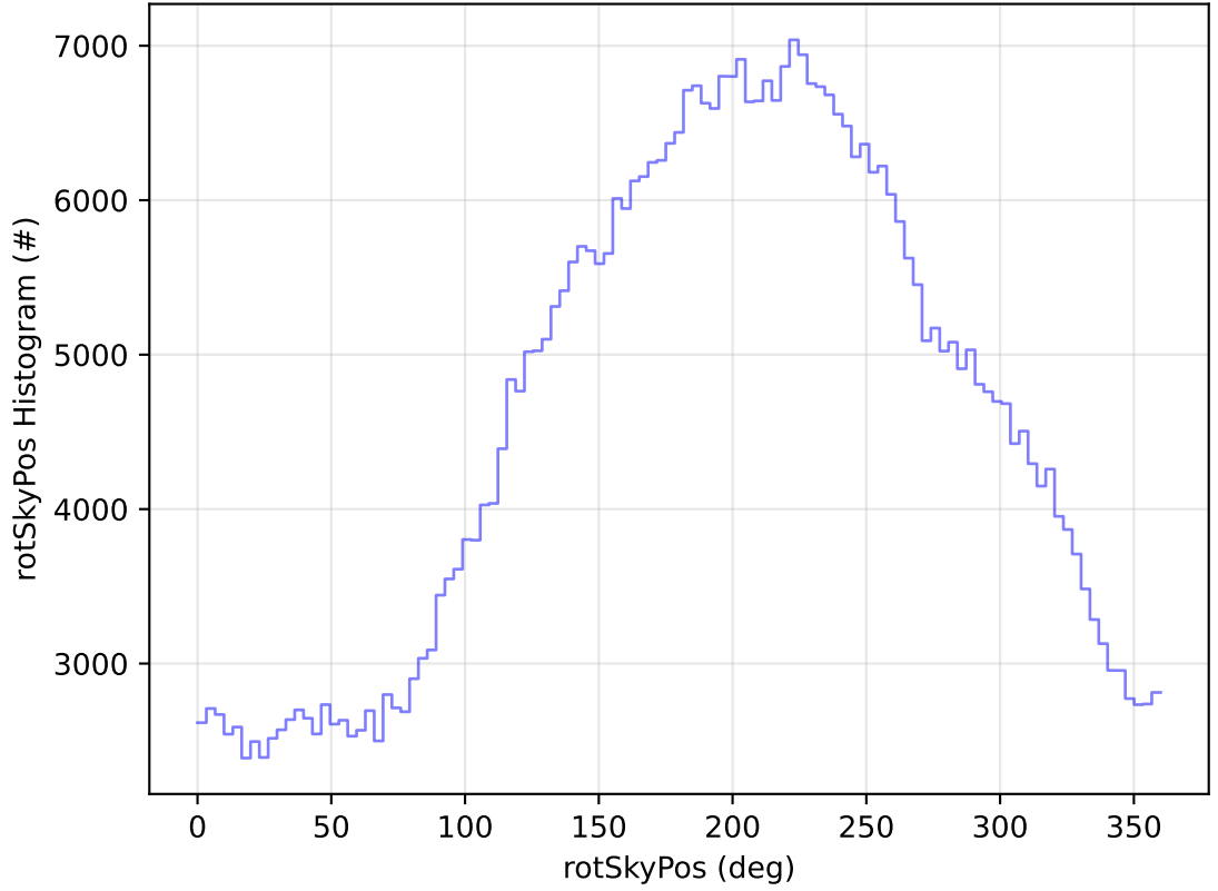
roll_uniform_early_half_mjdp0_v3.4_10yrs WFD i band: rotSkyPos Histogram
